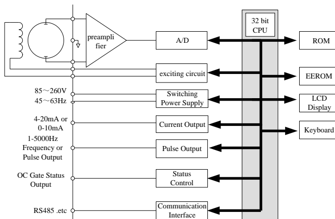
Fig.2. 1 Structure Of Converter's Circuit
