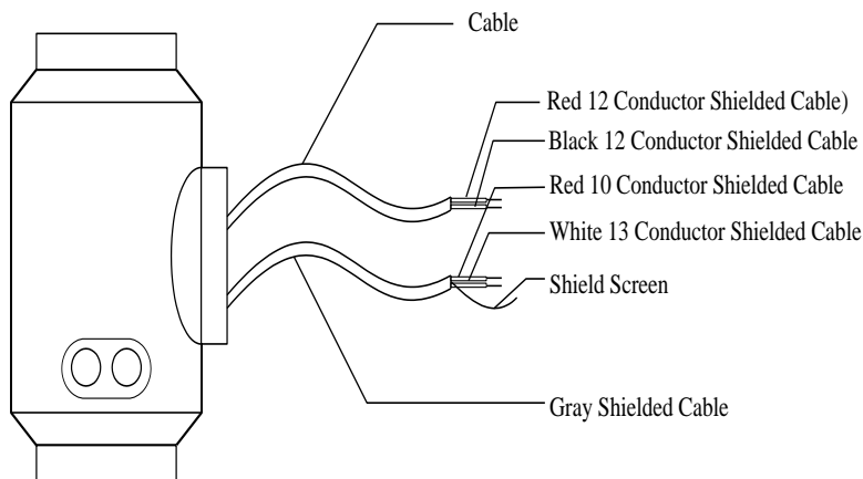
Fig.4.4.1 Labels and connection of signal lines in circinal model
