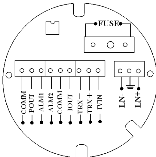
Fig.4.3 Connectors and labels
