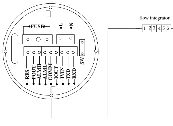
Fig 4.4.2(b) Connection of Electro-Mag 511Bnet Counter
