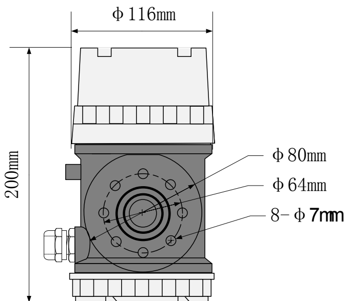
Fig.1.3 511B series 511C Shell
