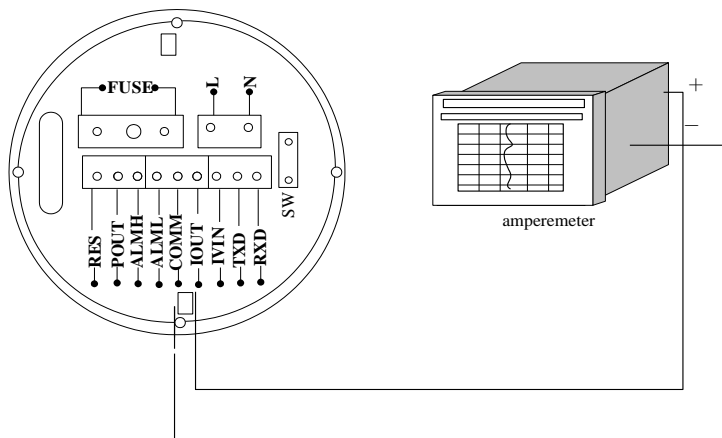
Fig 4.4.2(a) Output and power supply cables
