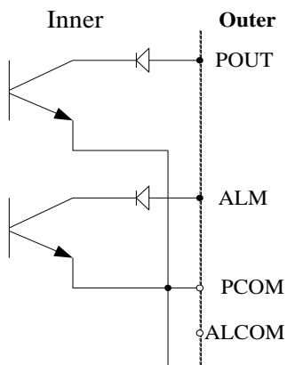
Fig.4.4.2(e) Connection of OC Gate
