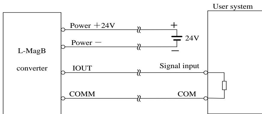
Fig.4.6 (c) L_Mag 511 four connection( power supply and current output are insulated)
