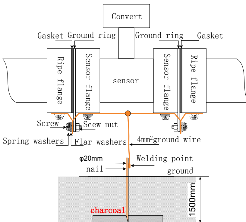
Fig.4.4.5 Grounding
