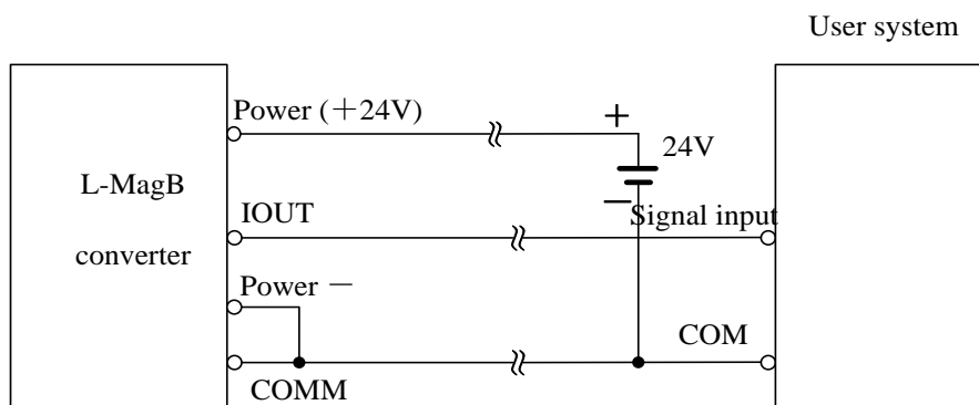
Fig.4.6 (b) L_Mag 511 three connection( power supply and current output are not insulated)
