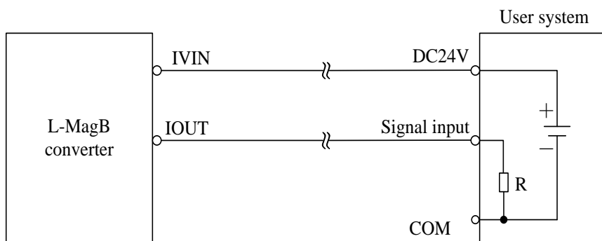
Fig.4.6 (a) L_Mag 511 two connection
